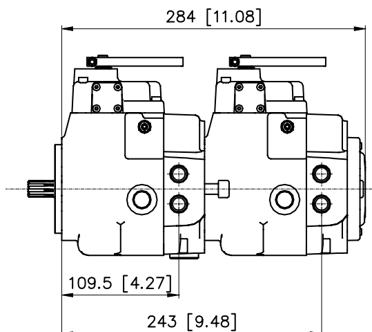
Alberi per pompe in tandem / Shafts for combination pumps
